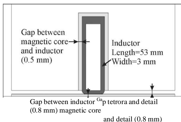
Figure 4. Induction system cross-section scheme.
