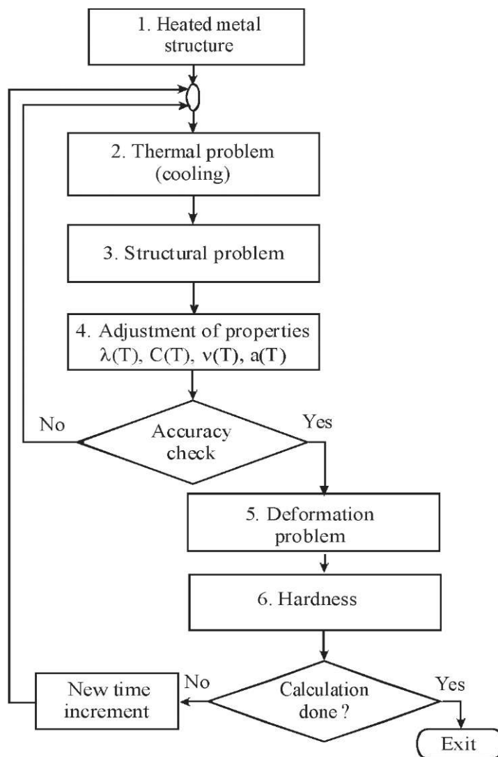
Figure 2. Modeling of the cooling process algorithm.
